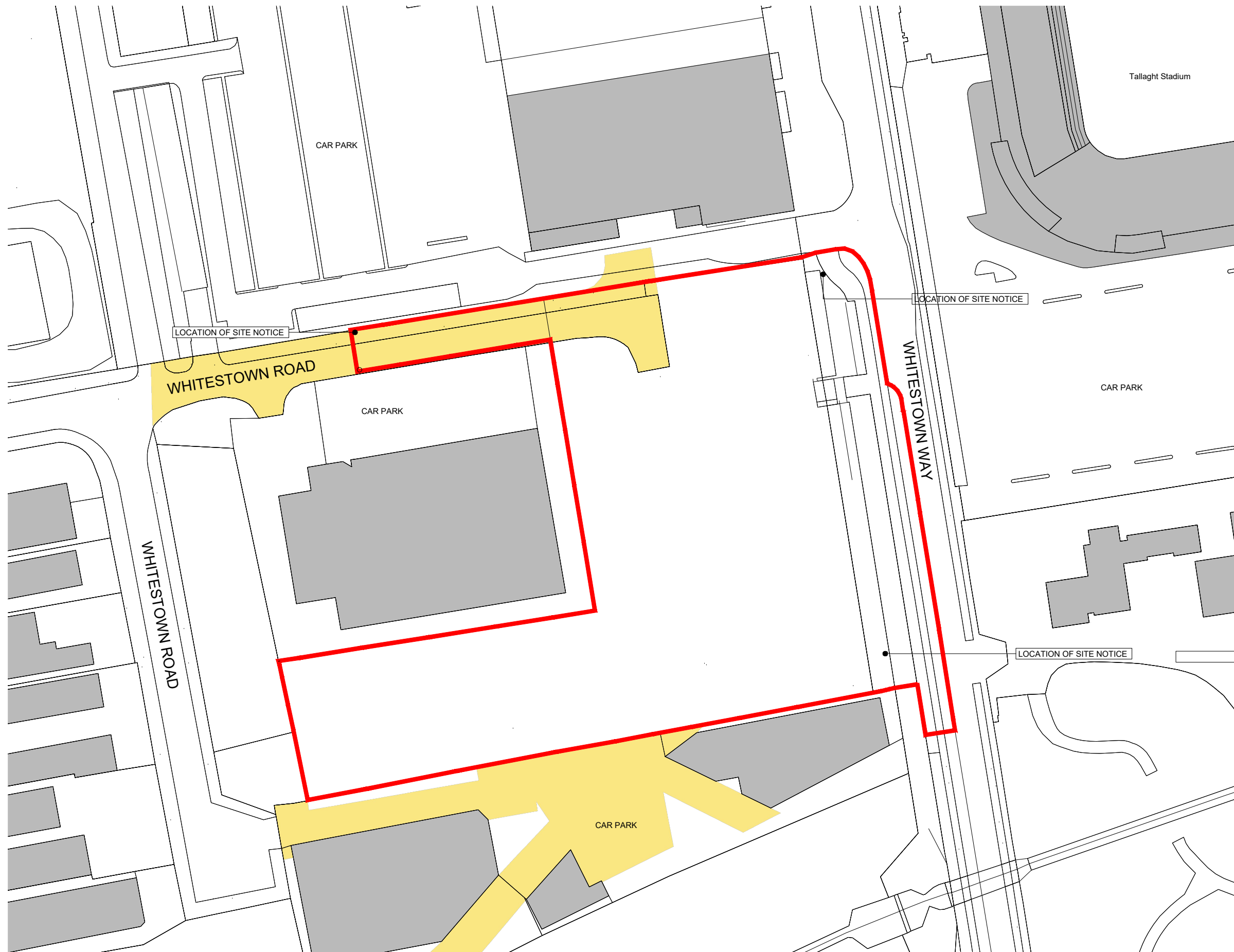
Site Location Plan 1:1000
