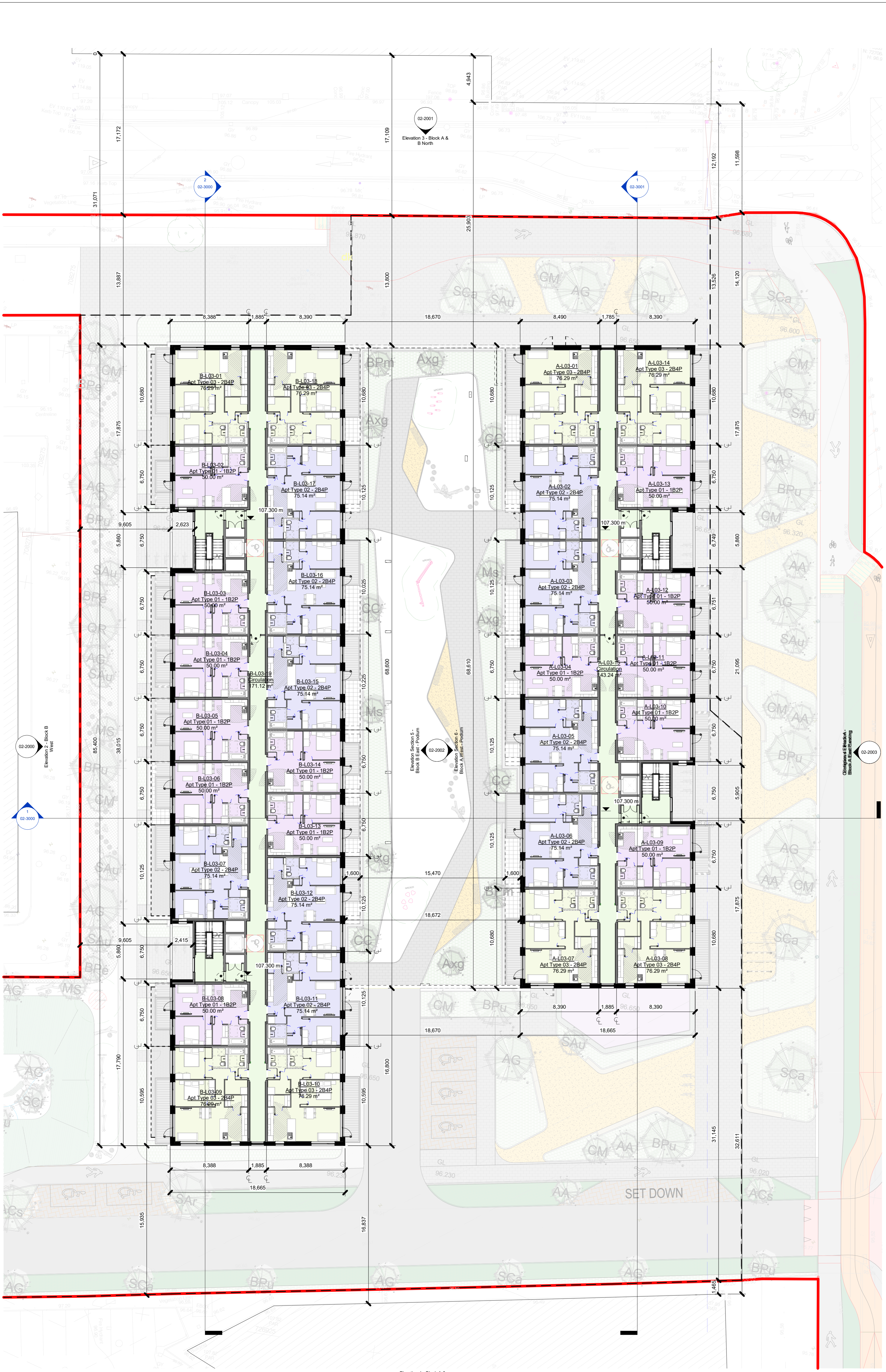
L03 - Proposed Third Floor Plan 1 : 200
