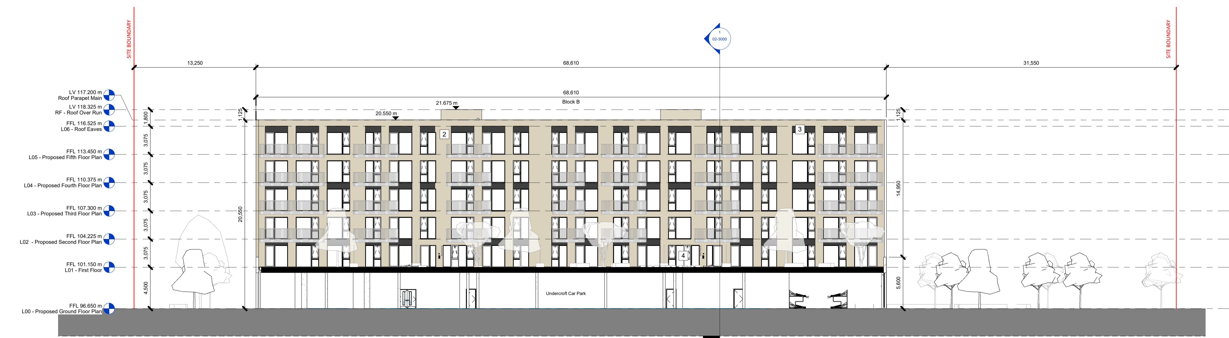
Elevation Section 6 - Block A West - Podium 1 : 200
