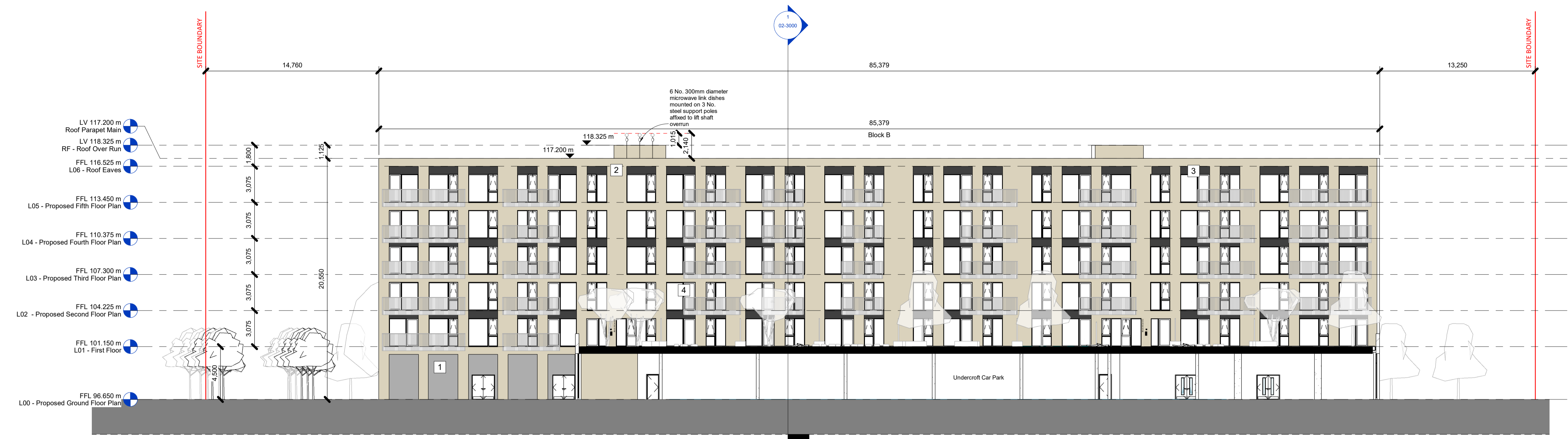
Elevation Section 5 - Block B East - Podium 1 : 200
